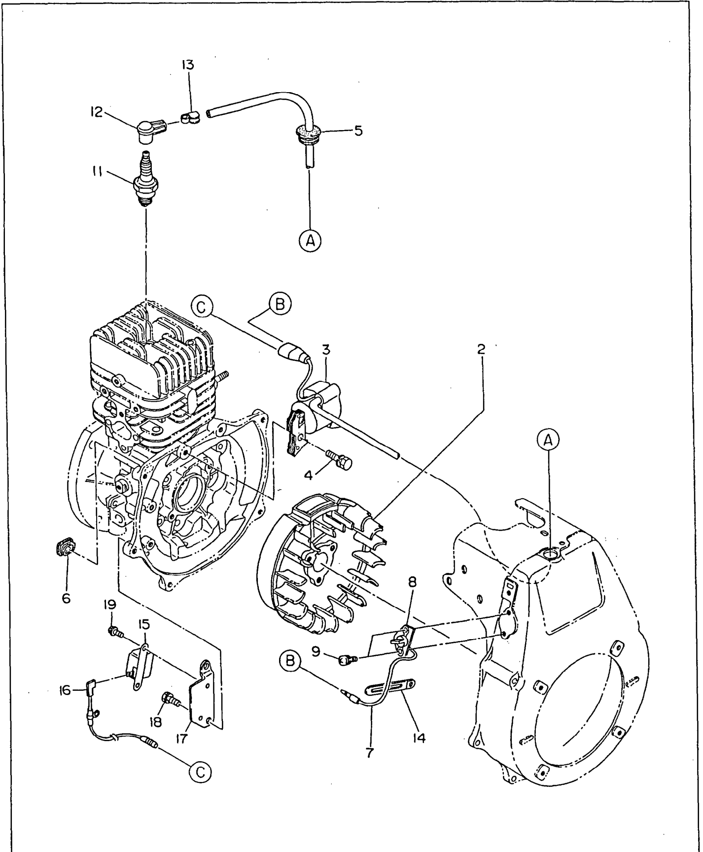
FIG. 5 ELECTRIC DEVICE
